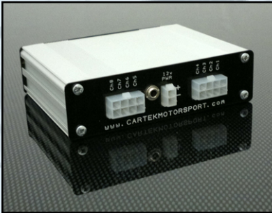
Relay Module (rear view)
